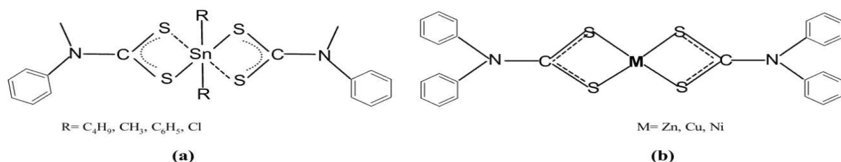
Figure 3. Chemical structure of (a) organotin(IV) N-methyl-N-phenyldithiocarbamate compounds, (b) Ni[S_2CN(C_6H_5)_2] , Zn[S_2CN(C_6H_5)_2] , and Cu[S_2CN(C_6H_5)_2]
