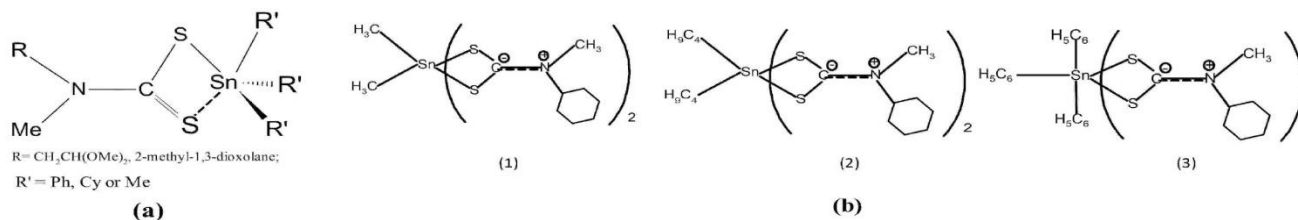
Figure 2. Structure of (a) [SnPh_3\{S_2CNR(R')\}]_n , [SnCy_3\{S_2CNR(R')\}]_n , [SnMe_3\{S_2CNR(R')\}]_n , [SnPh_3\{S_2CNR(R')\}]_n and [SnCy_3\{S_2CNR(R')\}]_n ; (b) Organotin(IV) dithiocarbamate compounds.
